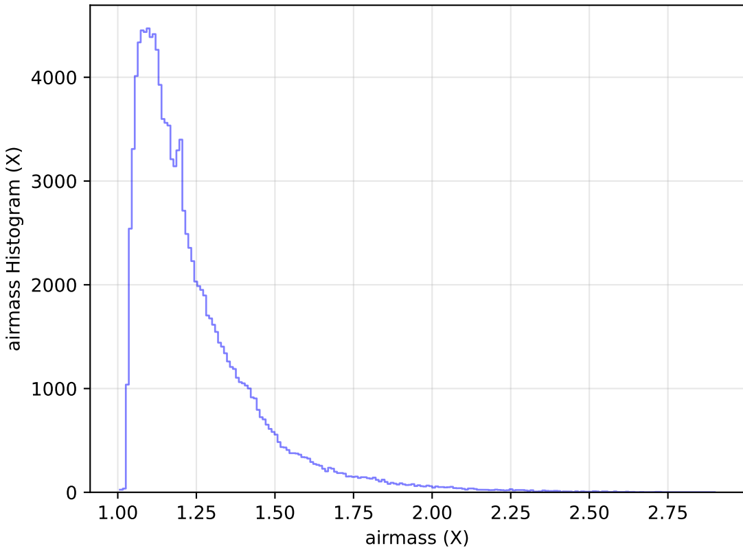
ddf_acor_sf10_lsf30_lsr20_v3.4_10yrs WFD u band: airmass Histogram
