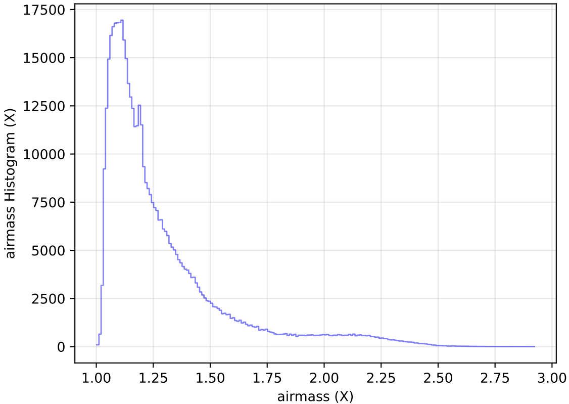
ddf_acor_sf10_lsf30_lsr20_v3.4_10yrs WFD r band: airmass Histogram
