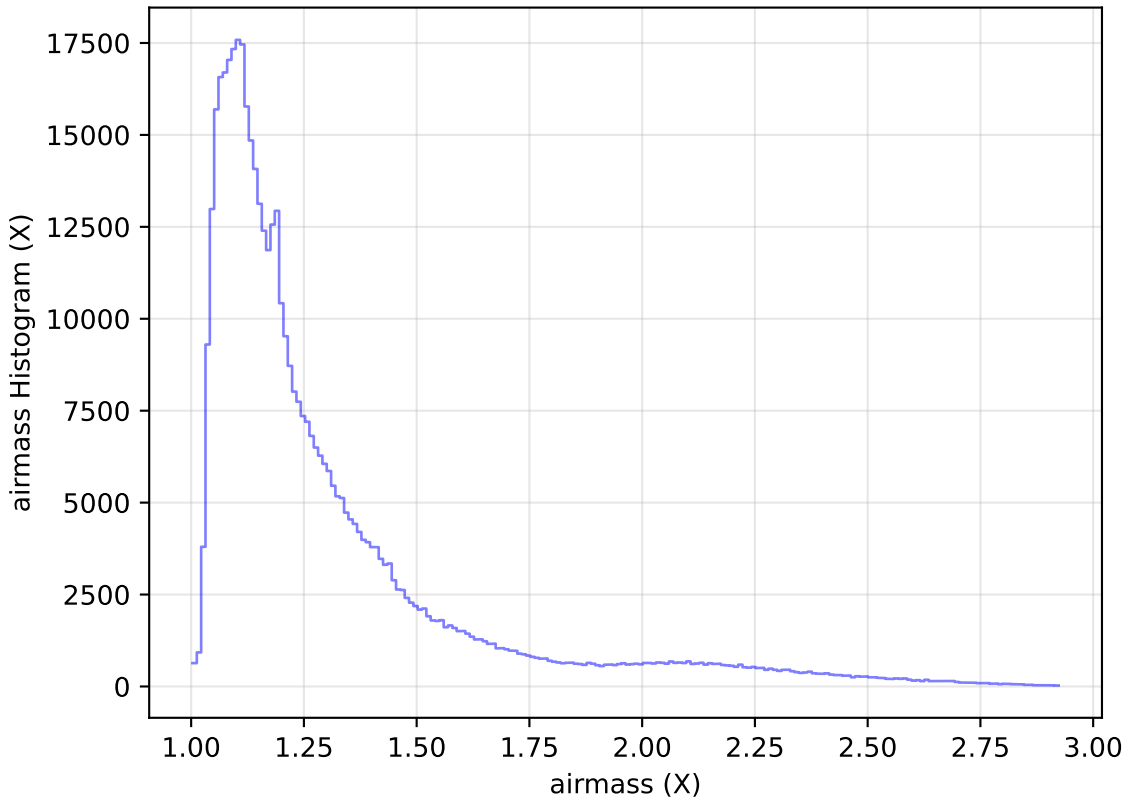
ddf_acor_sf10_lsf30_lsr20_v3.4_10yrs WFD i band: airmass Histogram
