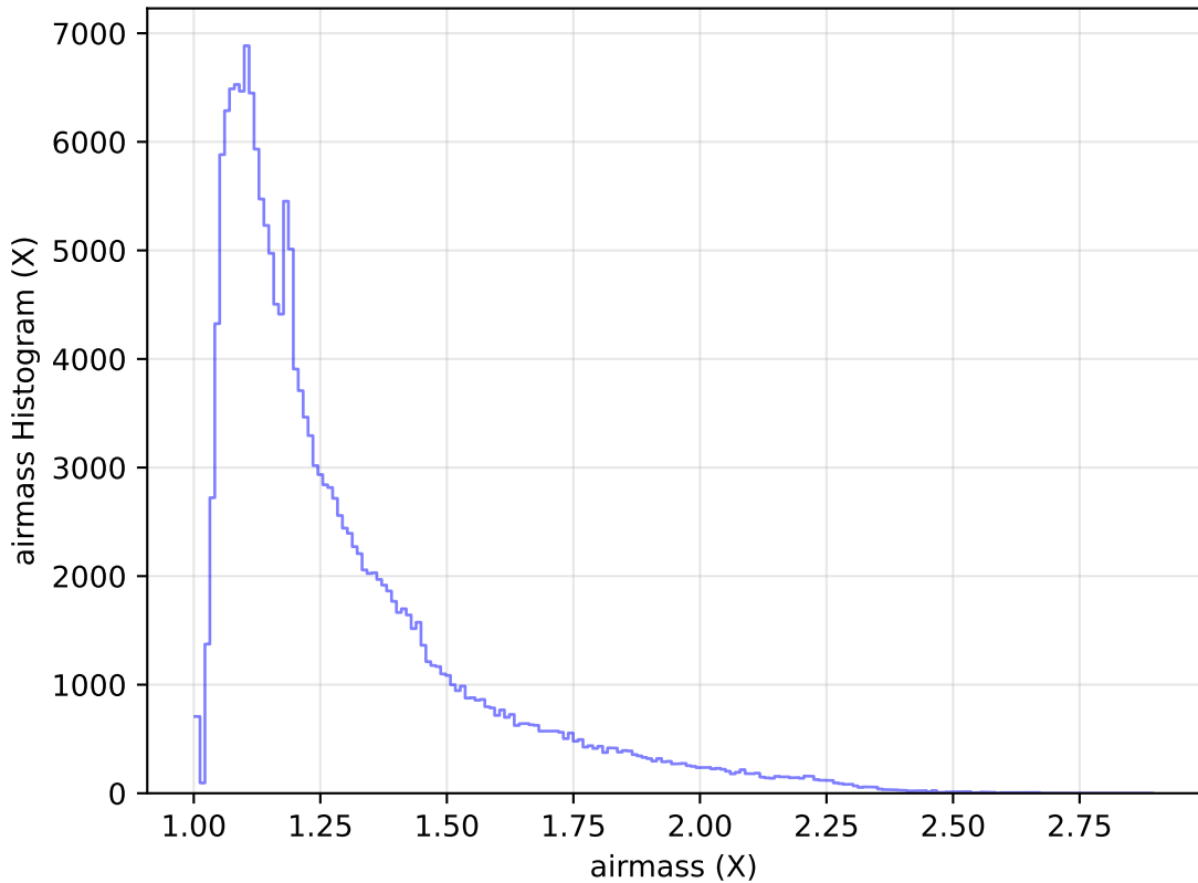
ddf_acor_sf10_lsf30_lsr20_v3.4_10yrs WFD g band: airmass Histogram
