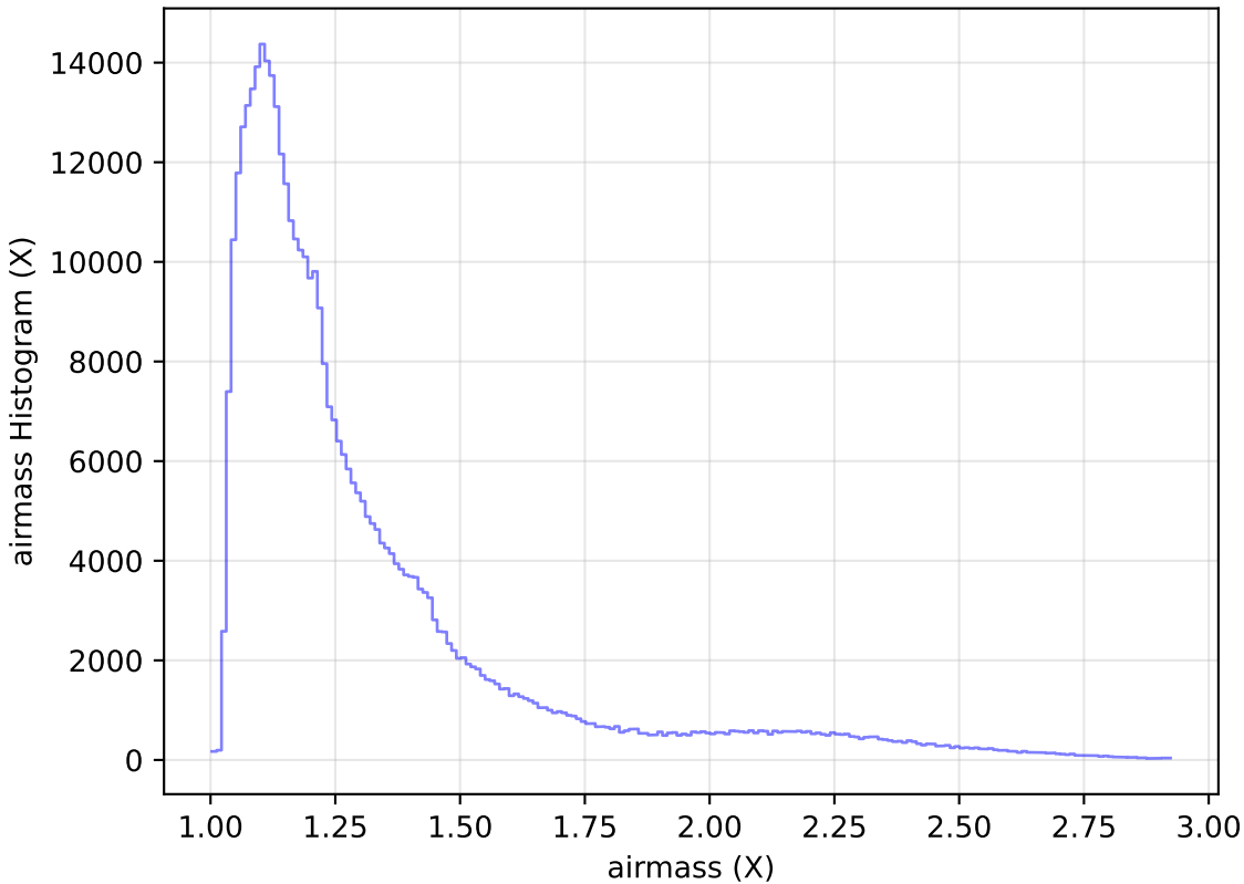
ddf_acor_sf10_lsf30_lsr20_v3.4_10yrs All sky z band: airmass Histogram
