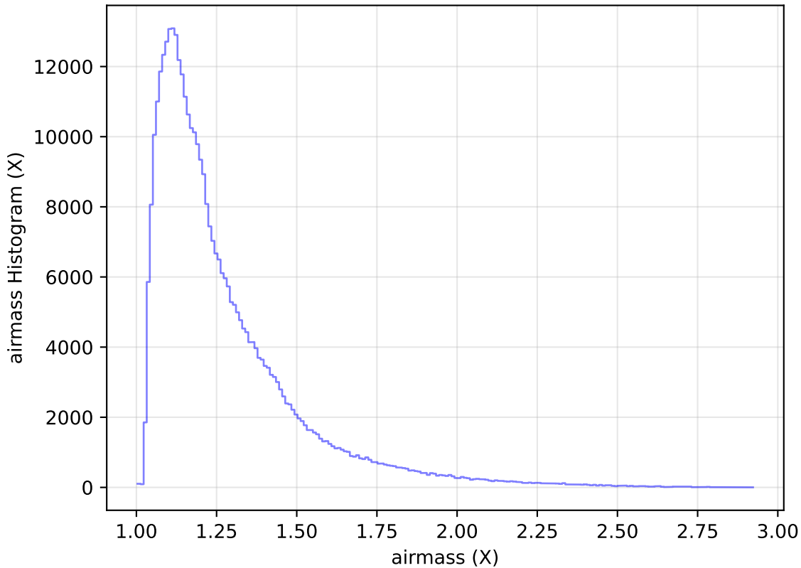
ddf_acor_sf10_lsf30_lsr20_v3.4_10yrs All sky y band: airmass Histogram
