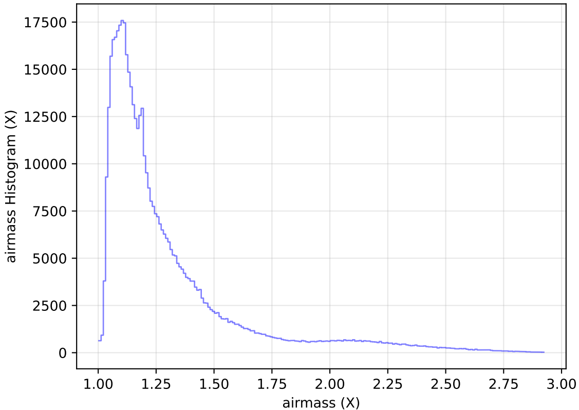
ddf_acor_sf10_lsf30_lsr20_v3.4_10yrs All sky i band: airmass Histogram
