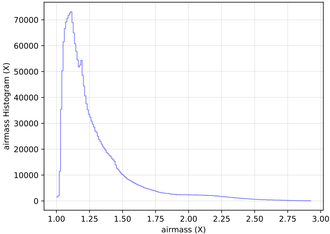
ddf_acor_sf10_lsf30_lsr20_v3.4_10yrs All sky all bands: airmass Histogram
