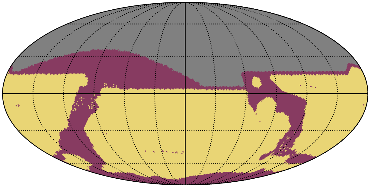
ddf_acor_sf10_lsf30_lsr20_v3.4_10yrs All sky: RapidRevisits
