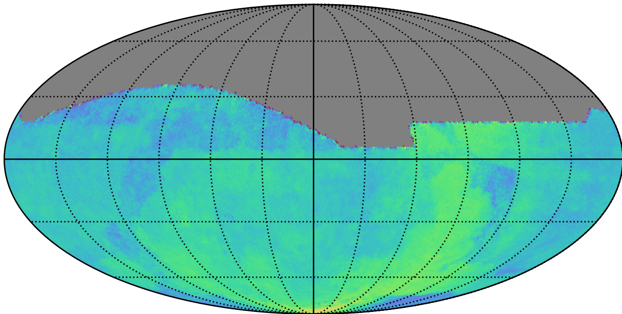
ddf_acor_sf10_lsf30_lsr20_v3.4_10yrs All sky: Parallax Coverage @ 24.0
