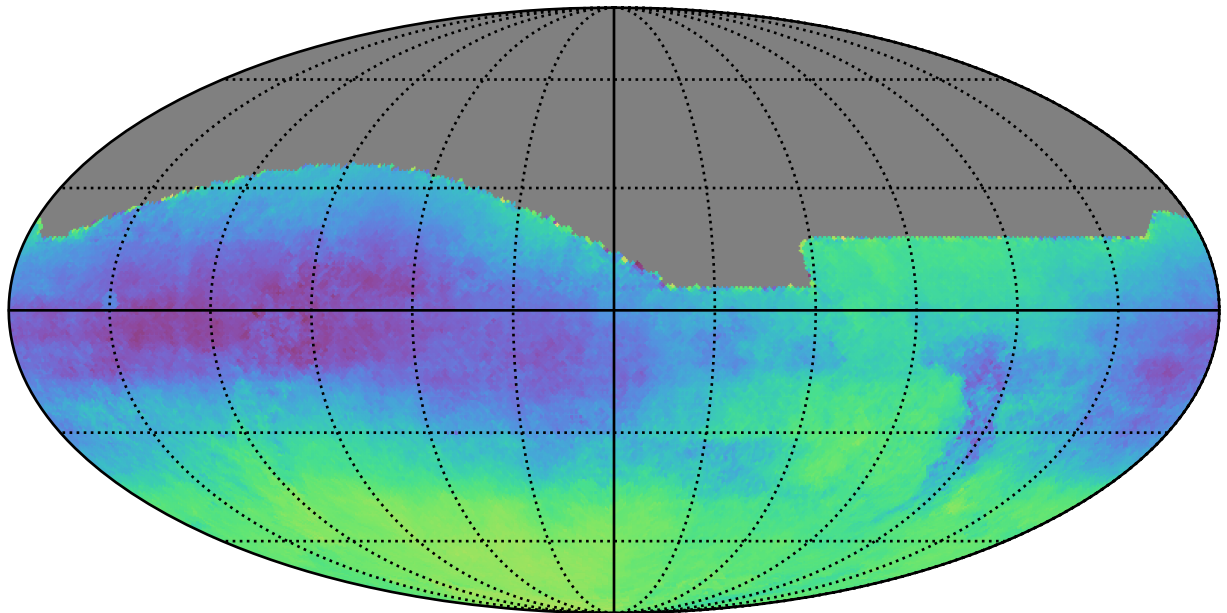
ddf_acor_sf10_lsf30_lsr20_v3.4_10yrs All sky: Parallax-DCR degeneracy @ 24.0
