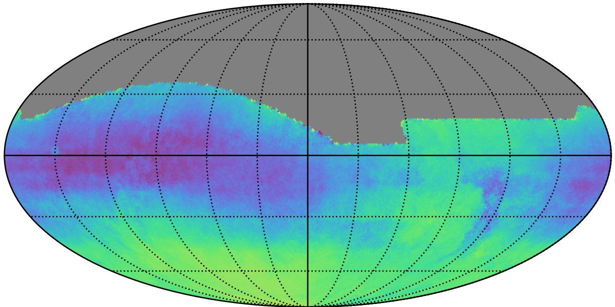
ddf_acor_sf10_lsf30_lsr20_v3.4_10yrs All sky: Parallax-DCR degeneracy @ 22.4
