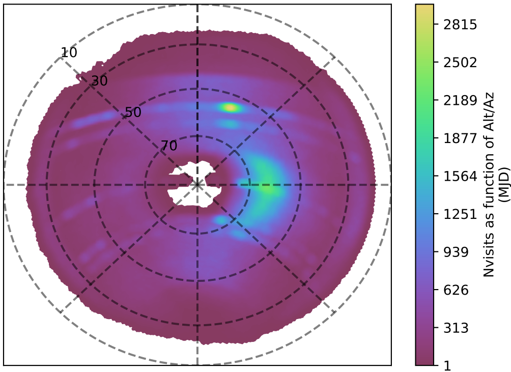
ddf_acor_sf10_lsf30_lsr20_v3.4_10yrs z band: Nvisits as function of Alt/Az
