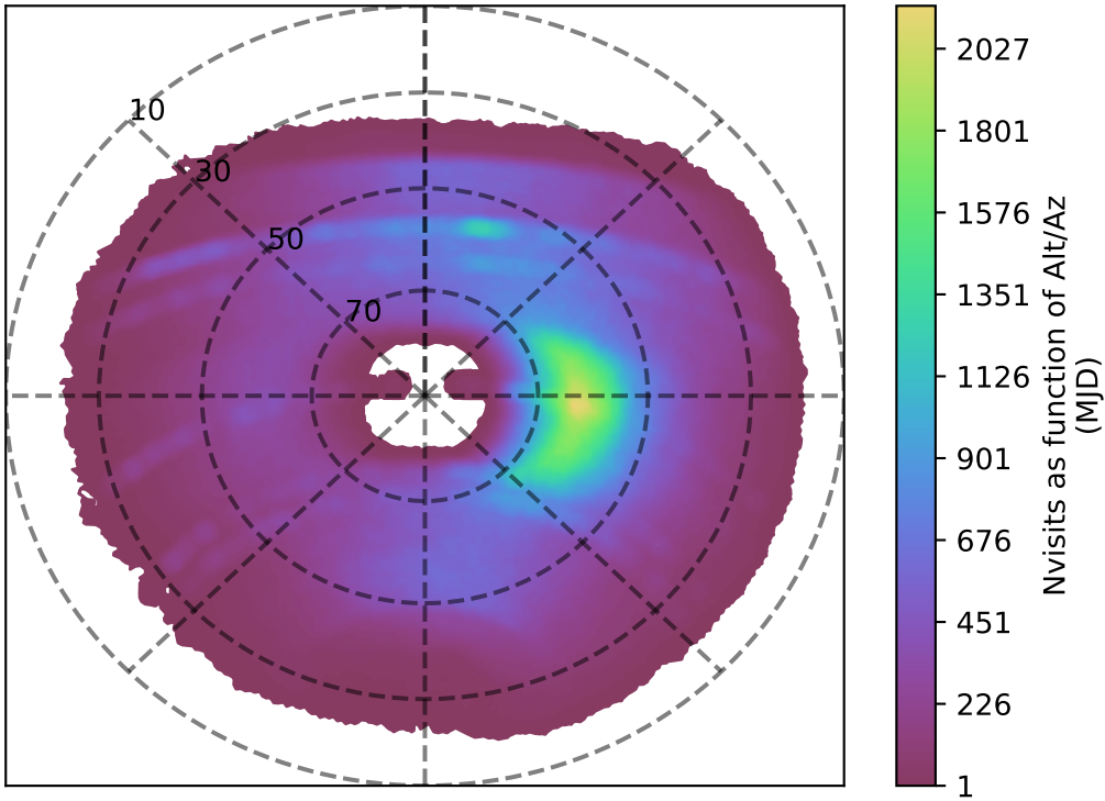
ddf_acor_sf10_lsf30_lsr20_v3.4_10yrs y band: Nvisits as function of Alt/Az
