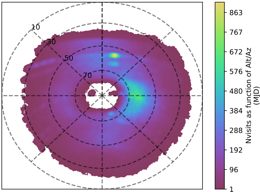
ddf_acor_sf10_lsf30_lsr20_v3.4_10yrs u band: Nvisits as function of Alt/Az
