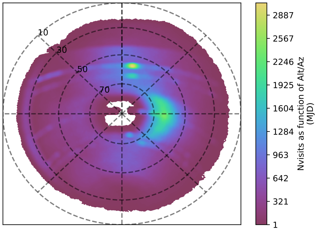
ddf_acor_sf10_lsf30_lsr20_v3.4_10yrs r band: Nvisits as function of Alt/Az
