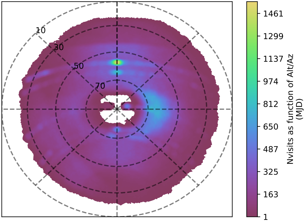
ddf_acor_sf10_lsf30_lsr20_v3.4_10yrs g band: Nvisits as function of Alt/Az
