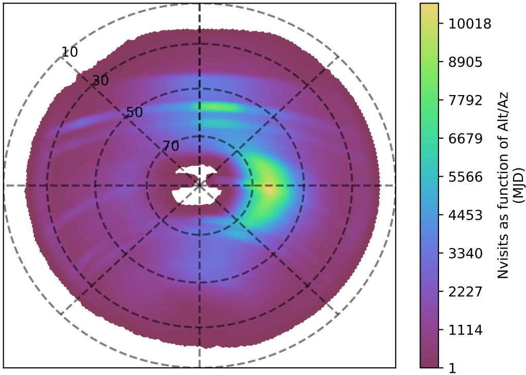
ddf_acor_sf10_ls30_lsr20_v3.4_10yrs all bands: Nvisits as function of Alt/Az
