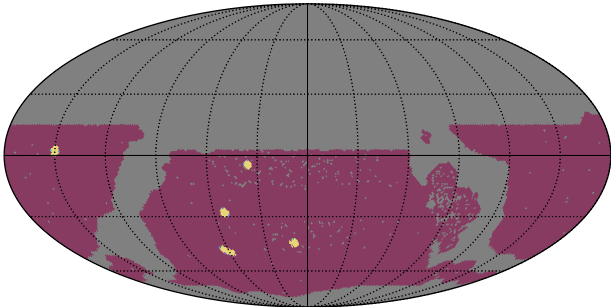
ddf_acor_sf10_lsf30_lsr20_v3.4_10yrs WFD: NumberOfQuickRevisits
