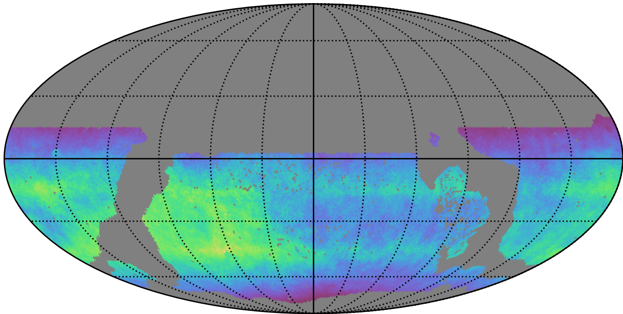
ddf_acor_sf10_lsf30_lsr20_v3.4_10yrs WFD i band: Normalized Teff
