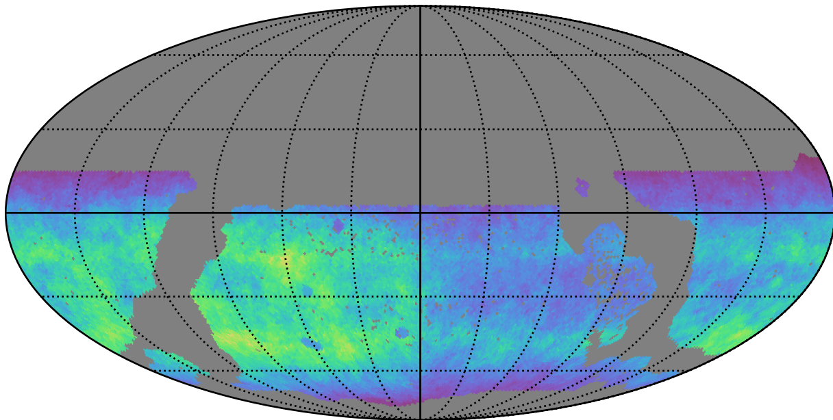
ddf_acor_sf10_lsf30_lsr20_v3.4_10yrs WFD g band: Normalized Teff
