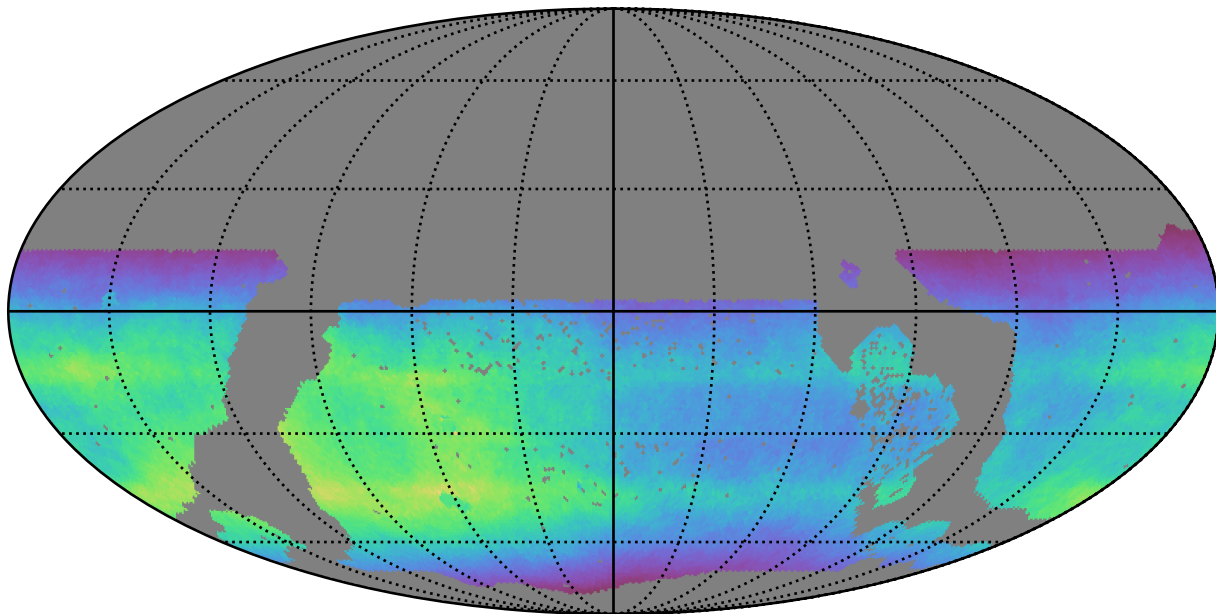
ddf_acor_sf10_lsf30_lsr20_v3.4_10yrs WFD all bands: Normalized Teff
