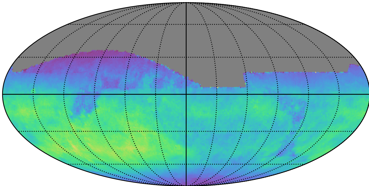
ddf_acor_sf10_lsf30_lsr20_v3.4_10yrs All sky z band: Normalized Teff
