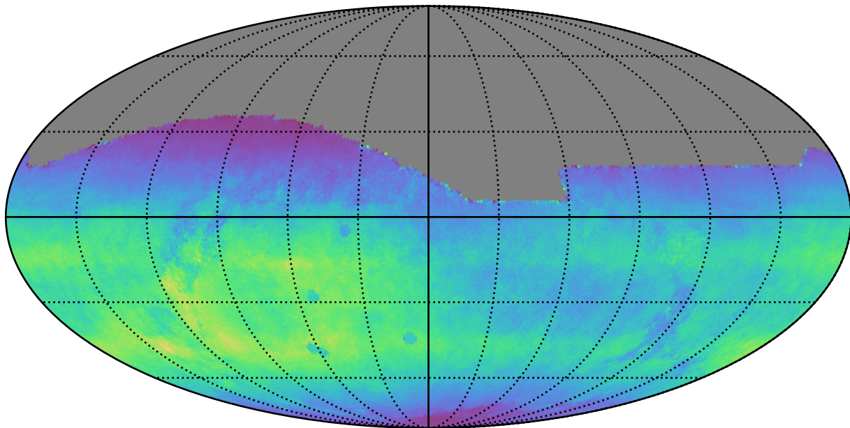
ddf_acor_sf10_lsf30_lsr20_v3.4_10yrs All sky r band: Normalized Teff
