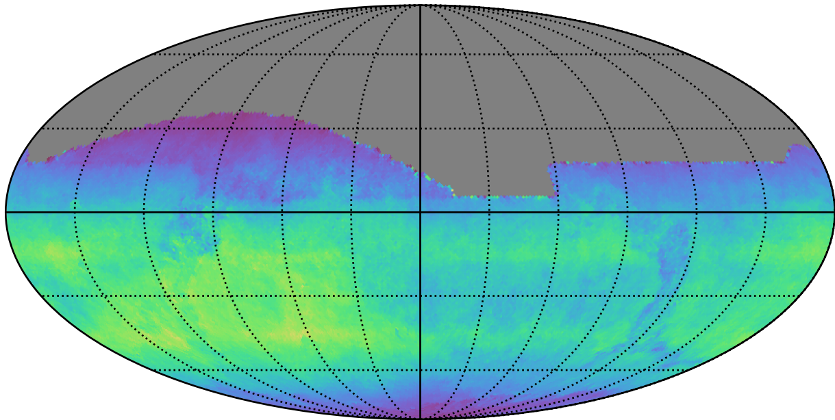
ddf_acor_sf10_lsf30_lsr20_v3.4_10yrs All sky i band: Normalized Teff
