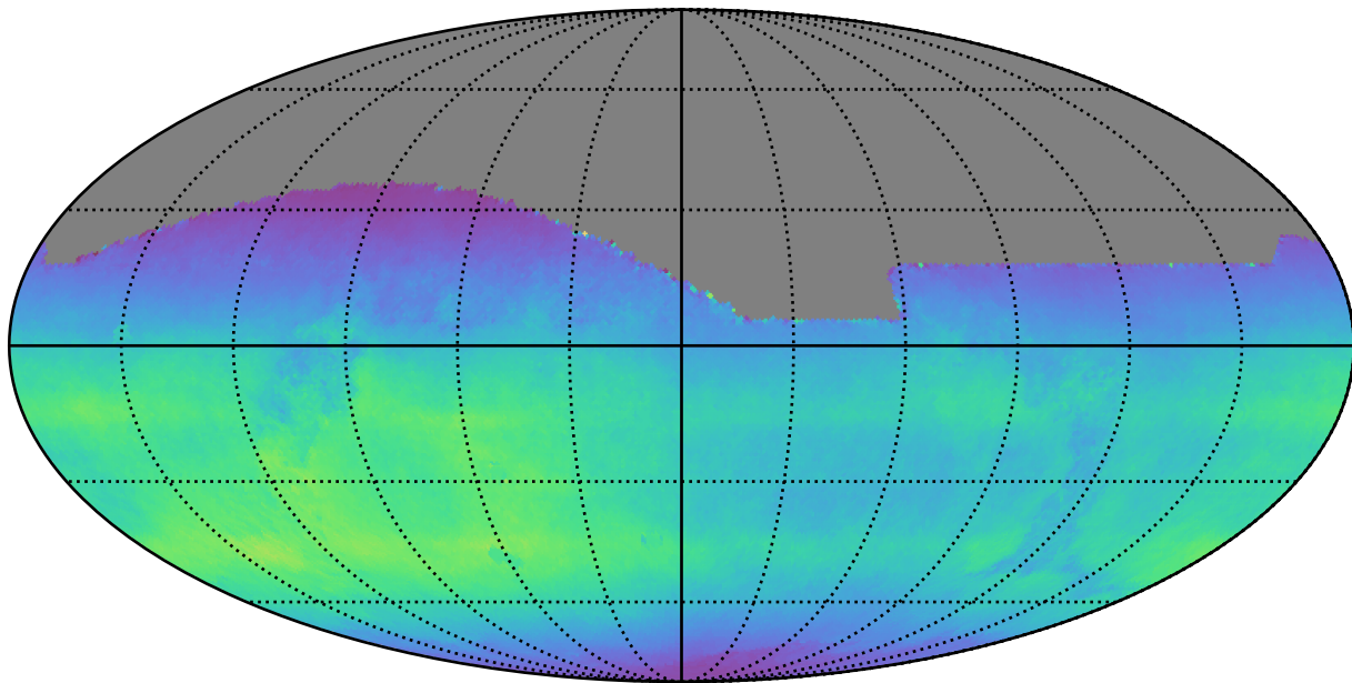
ddf_acor_sf10_lsf30_lsr20_v3.4_10yrs All sky all bands: Normalized Teff
