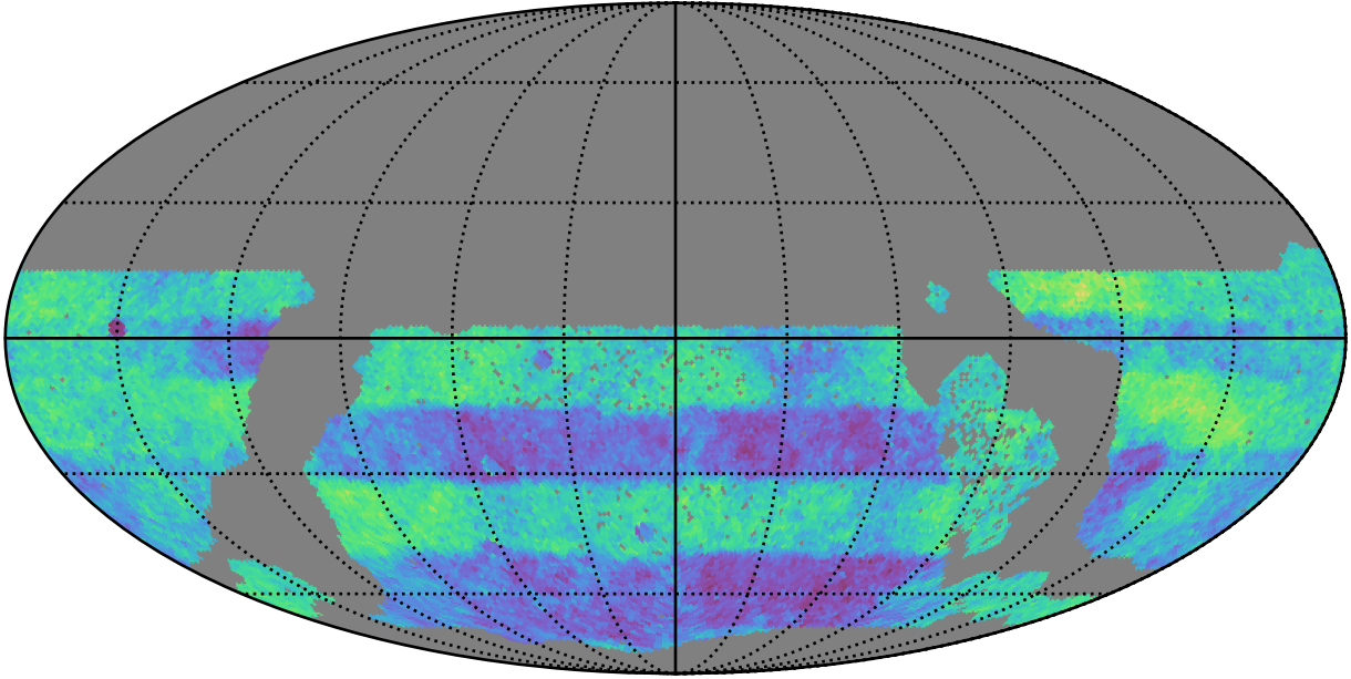
ddf_acor_sf10_lsf30_lsr20_v3.4_10yrs WFD: Normalized Proper Motion Uncert @ 24.0
