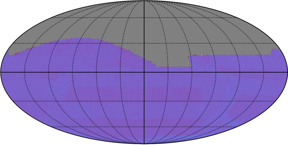
ddf_acor_sf10_lsf30_lsr20_v3.4_10yrs All sky: Normalized Proper Motion Uncert @ 20.5
