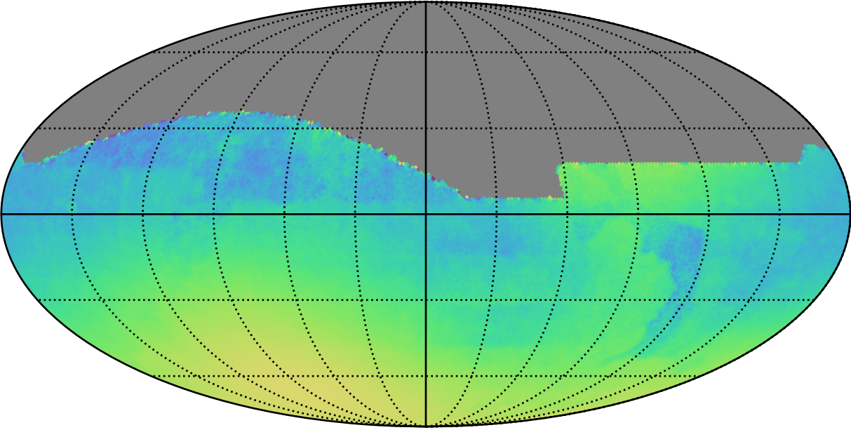
ddf_acor_sf10_lsf30_lsr20_v3.4_10yrs All sky: Normalized Parallax Uncert @ 22.4
