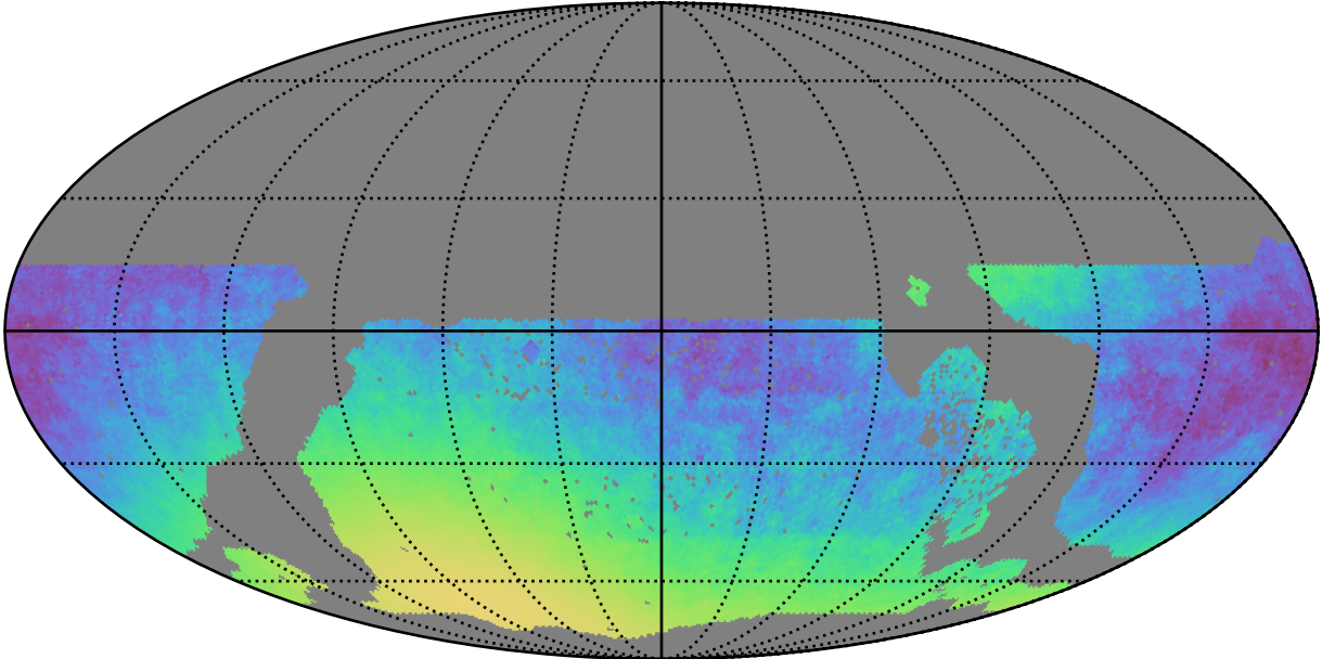
ddf_acor_sf10_lsf30_lsr20_v3.4_10yrs WFD y band only: Normalized Parallax Uncert @ 21.3
