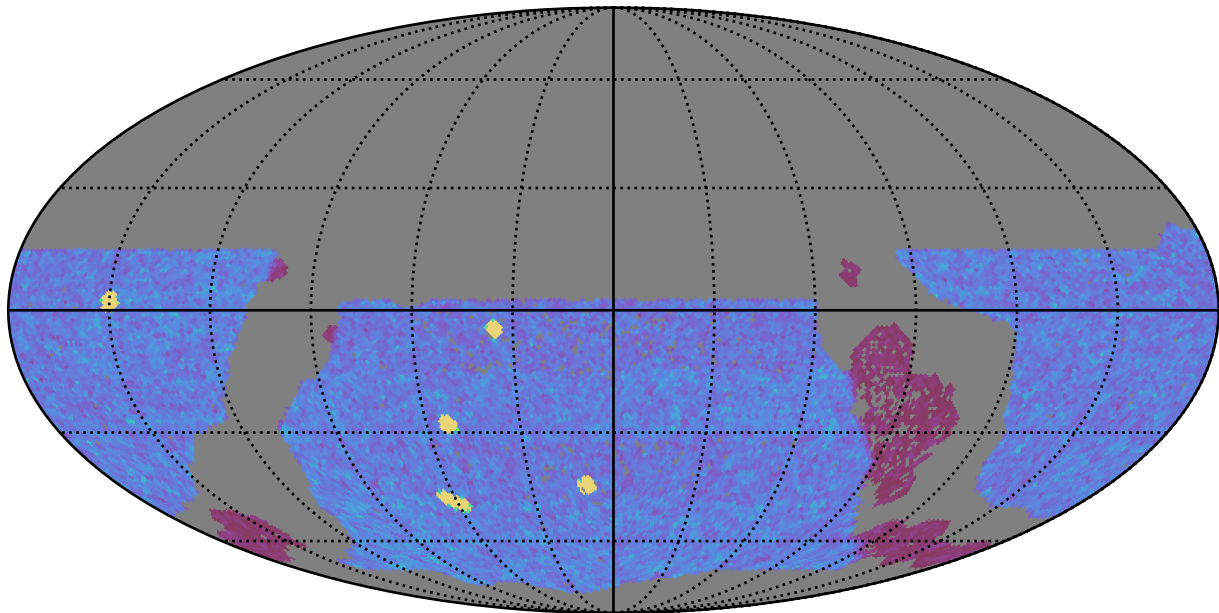
ddf_acor_sf10_lsf30_lsr20_v3.4_10yrs WFD y band: NVisits
