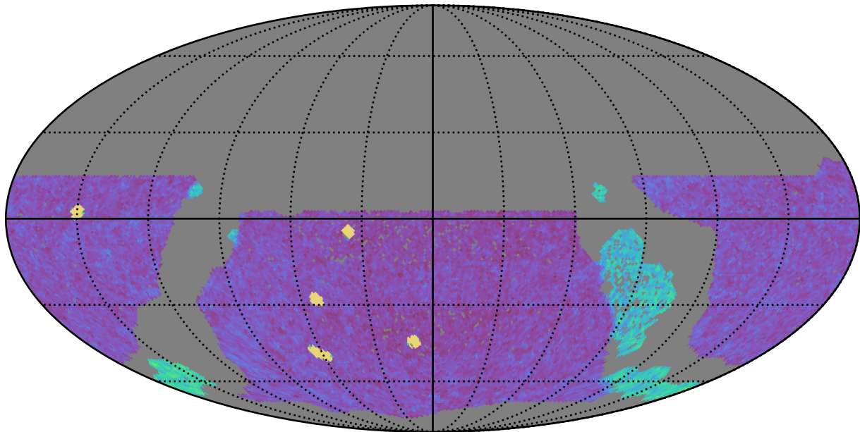
ddf_acor_sf10_lsf30_lsr20_v3.4_10yrs WFD g band: NVisits
