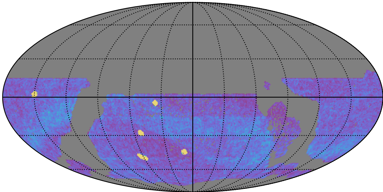
ddf_acor_sf10_lsf30_lsr20_v3.4_10yrs WFD all bands: NVisits
