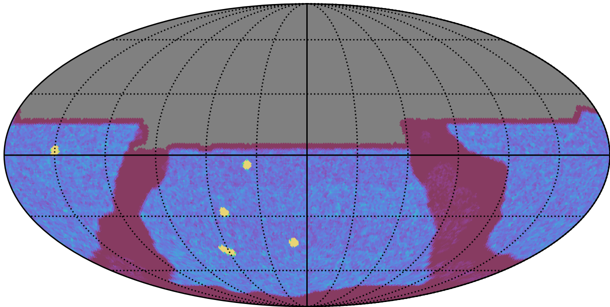
ddf_acor_sf10_lsf30_lsr20_v3.4_10yrs All sky y band: NVisits
