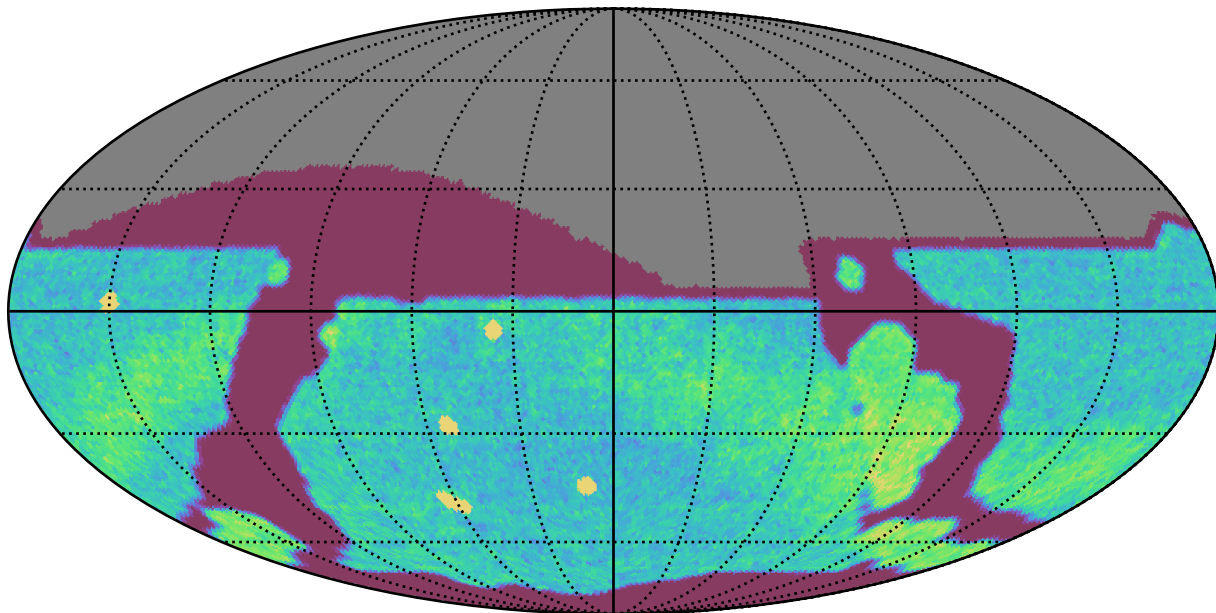
ddf_acor_sf10_lsf30_lsr20_v3.4_10yrs All sky r band: NVisits
