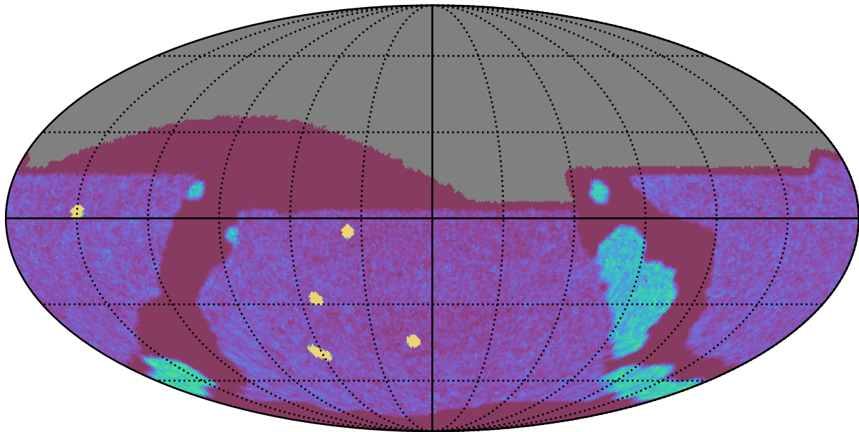
ddf_acor_sf10_lsf30_lsr20_v3.4_10yrs All sky g band: NVisits
