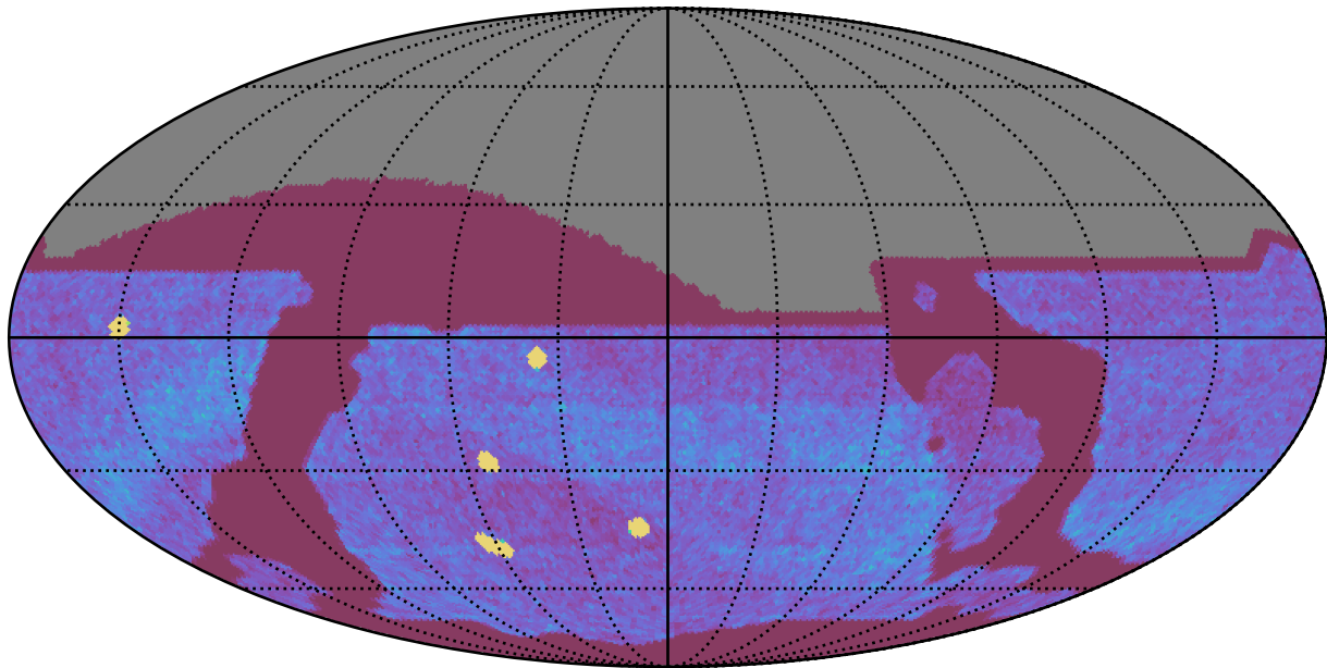
ddf_acor_sf10_lsf30_lsr20_v3.4_10yrs All sky all bands: NVisits
