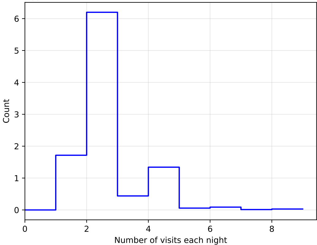
ddf_acor_sf10_lsf30_lsr20_v3.4_10yrs All sky: NVisitsPerNight 1e6
