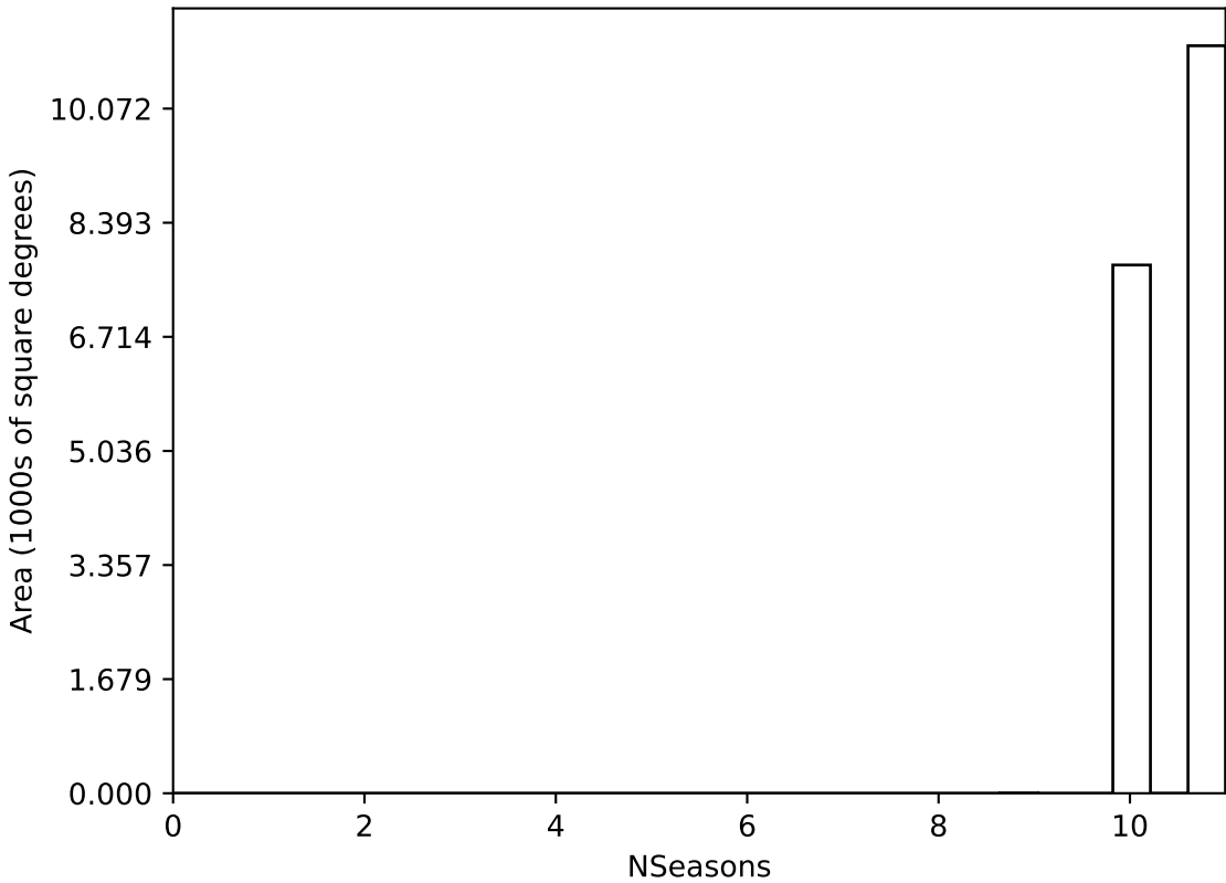
ddf_acor_sf10_lsf30_lsr20_v3.4_10yrs WFD all bands: NSeasons
