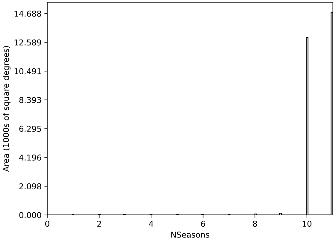
ddf_acor_sf10_lsf30_lsr20_v3.4_10yrs All sky all bands: NSeasons
