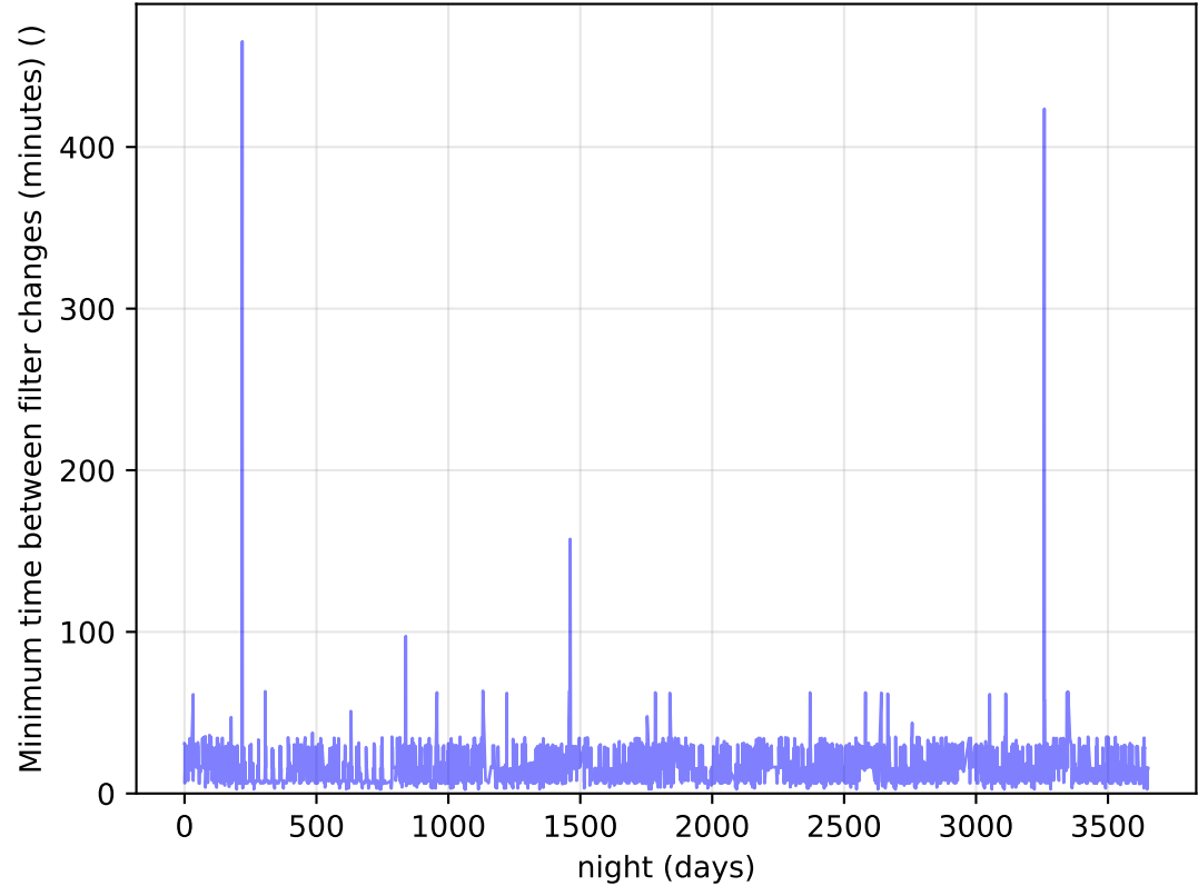
ddf_acor_sf10_Isf30_Isr20_v3.4_10yrs Per Night: Minimum time between filter changes (minutes)
