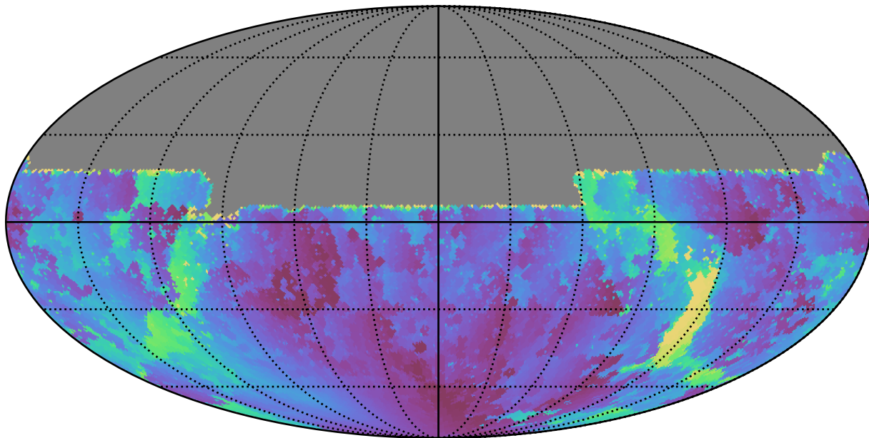
ddf_acor_sf10_lsf30_lsr20_v3.4_10yrs All sky u band: Min solarElong
