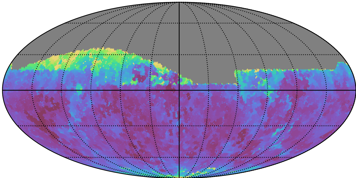
ddf_acor_sf10_lsf30_lsr20_v3.4_10yrs Yr 1 i band: Min seeingEff
