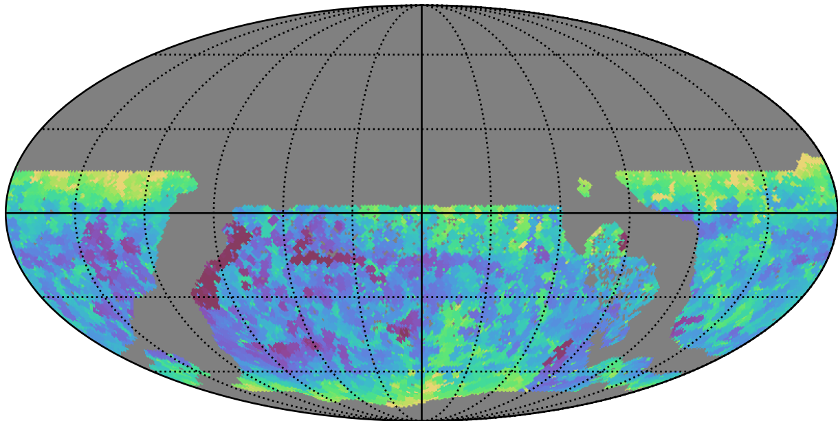
ddf_acor_sf10_lsf30_lsr20_v3.4_10yrs WFD y band: Min seeingEff
