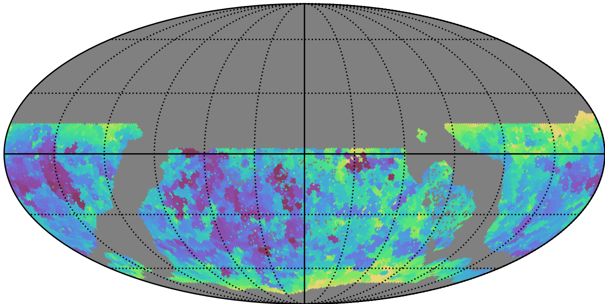
ddf_acor_sf10_lsf30_lsr20_v3.4_10yrs WFD g band: Min seeingEff
