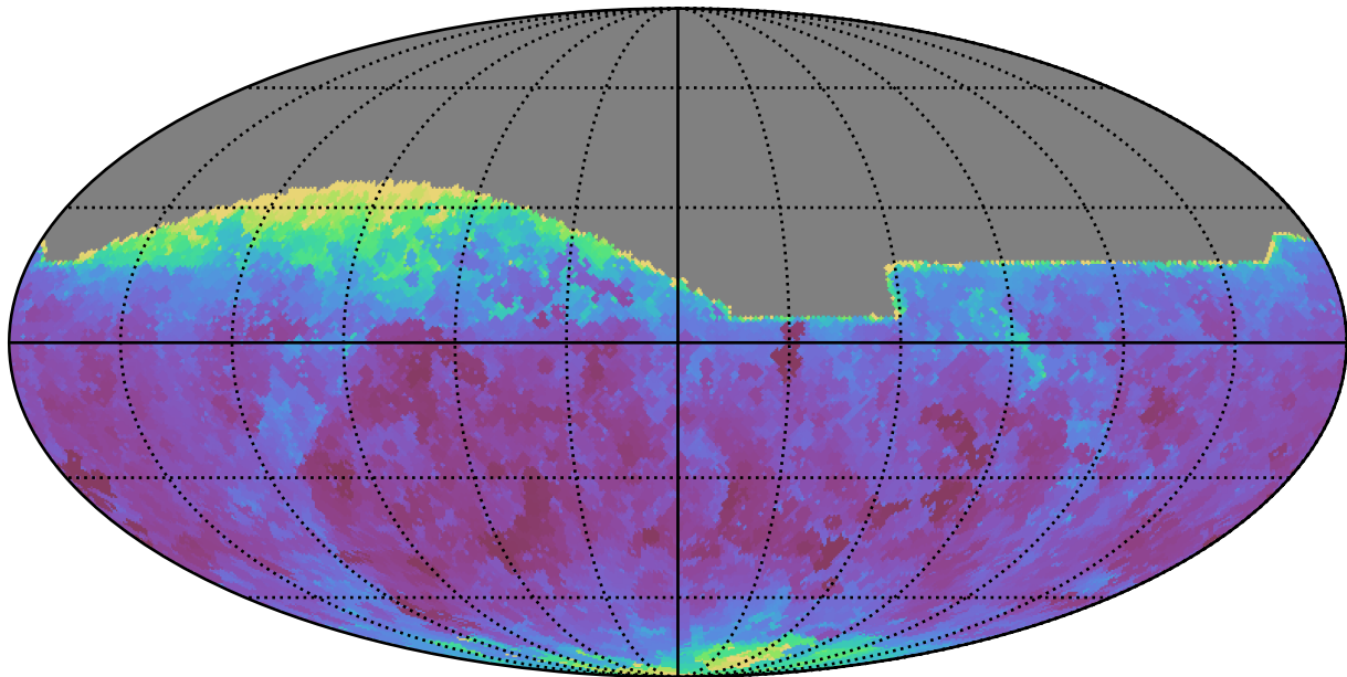
ddf_acor_sf10_lsf30_lsr20_v3.4_10yrs All sky z band: Min seeingEff
