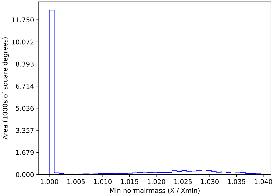
ddf_acor_sf10_lsf30_lsr20_v3.4_10yrs WFD y band: Min normairmass
