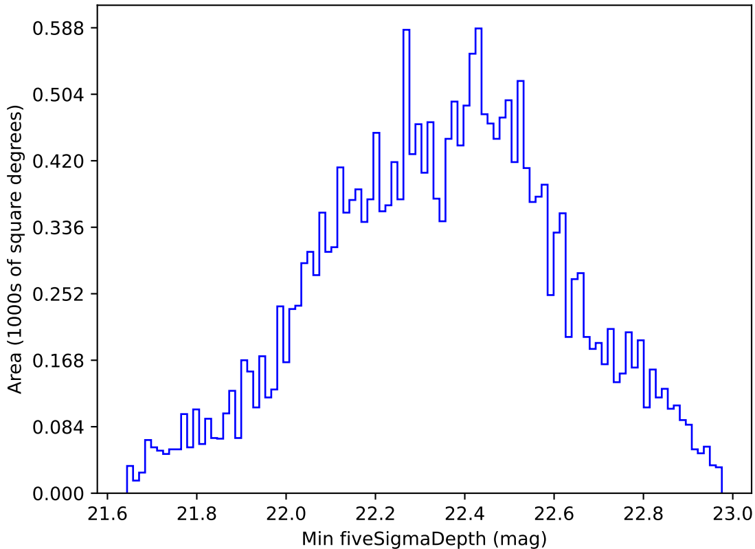
ddf_acor_sf10_lsf30_lsr20_v3.4_10yrs All sky u band: Min fiveSigmaDepth
