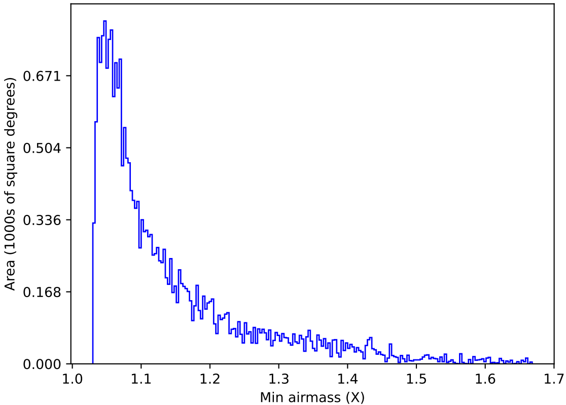
ddf_acor_sf10_lsf30_lsr20_v3.4_10yrs Yr 1 u band: Min airmass
