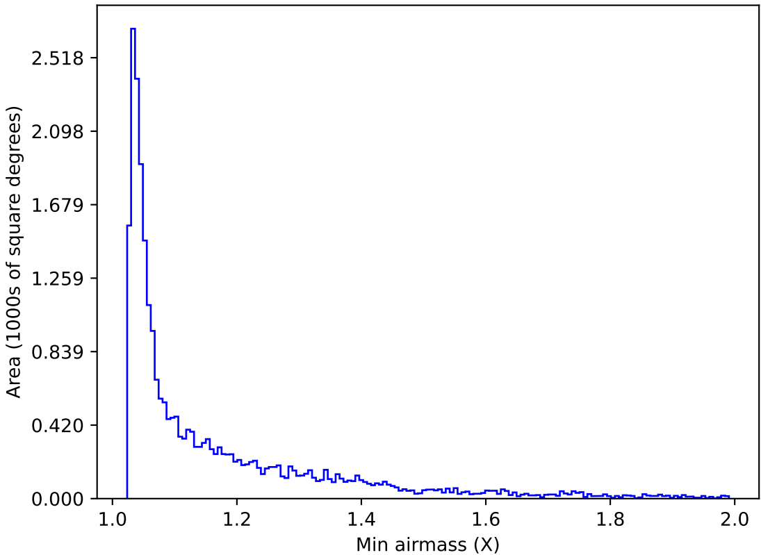
ddf_acor_sf10_lsf30_lsr20_v3.4_10yrs Yr 1 r band: Min airmass
